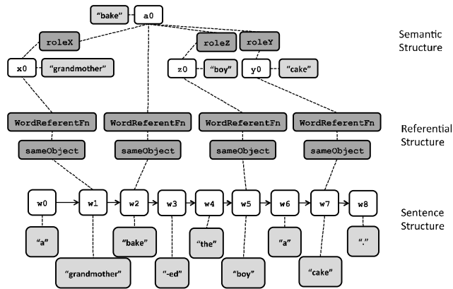
Figure 2: Interrelations between semantic and sentence structure through the referential structure layer.
